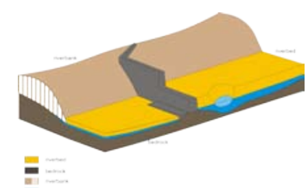
Figure 3: Riverbed with a sand storage dam during the dry season. Water availability is considerably larger compared to a river without a sand storage dam (Hoogmoed, 2009)
